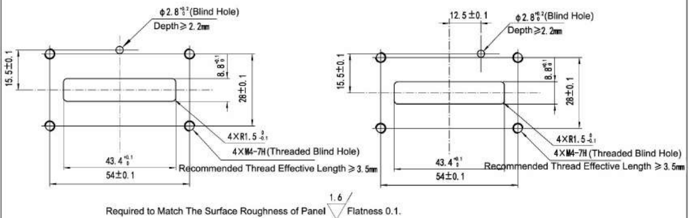
Recommended Panel Hole Size (Socket HCIL-F4P(16A)-A-1)
