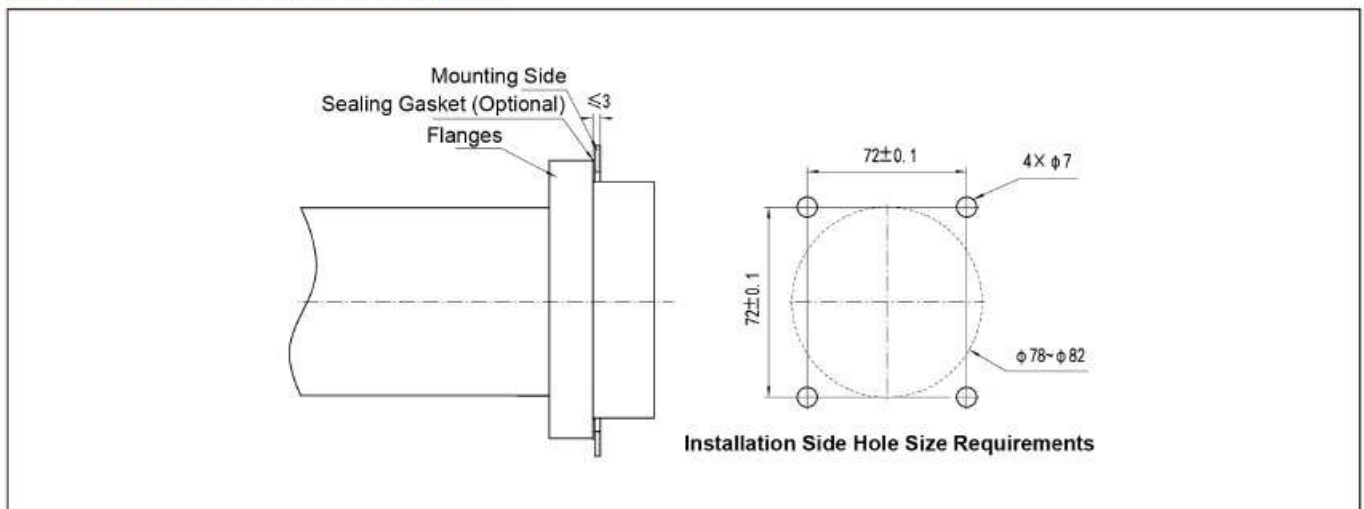
[DC Charging Socket Rear Mount Diagram]
