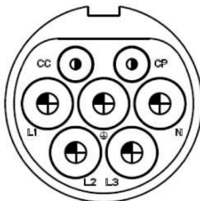
Contact Arrangement (Take the Gun As an Example)
