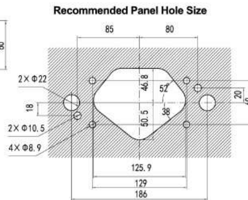
Fixed Plug
