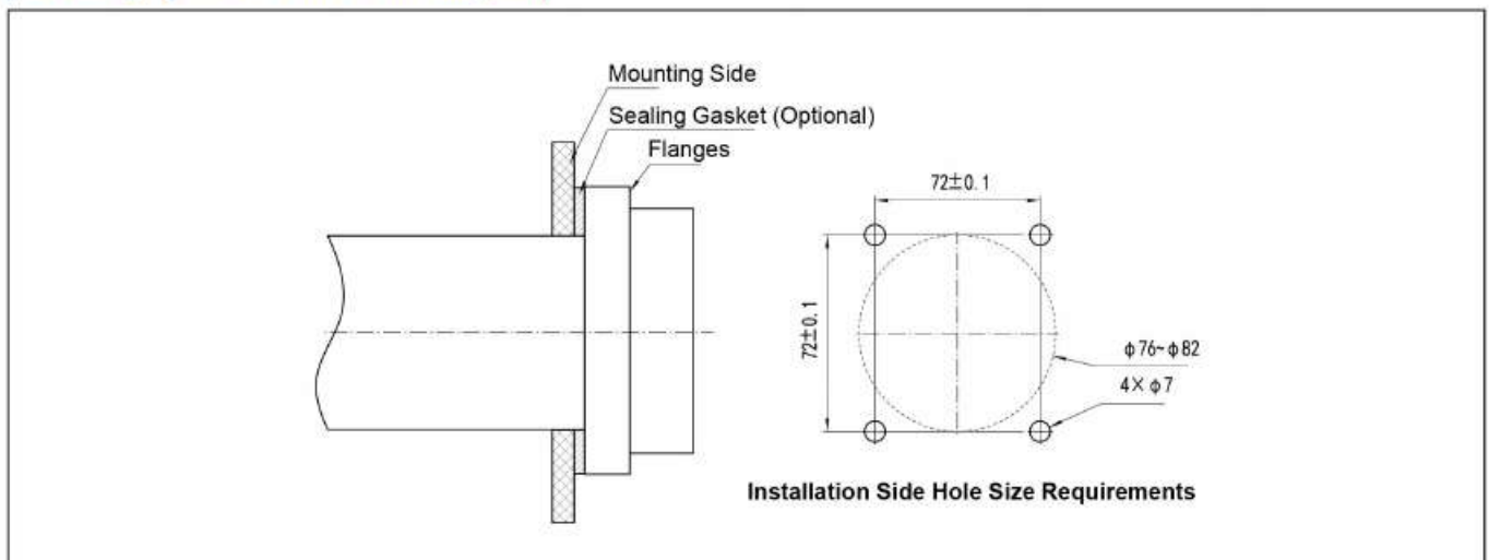
[DC Charging Socket Front Mount Diagram]
