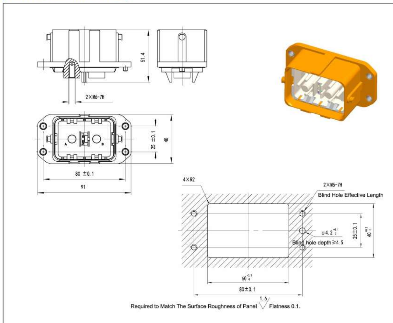
[Square Flange Socket HVIL-F2P(150A)]
